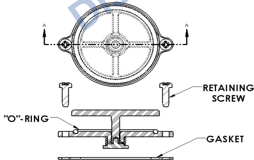
EQUALIZER VALVE ASSEMBLY SP1078
